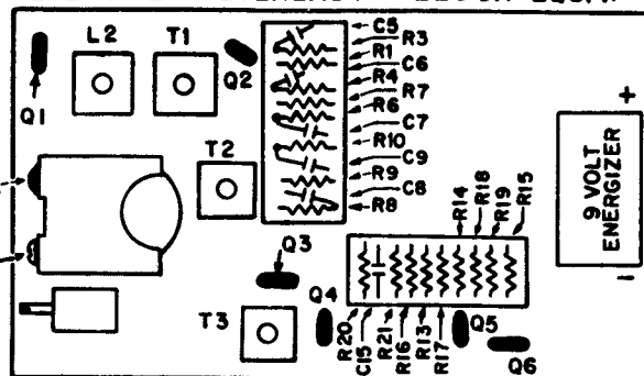
ALIGNMENT, TRANSISTOR AND BATTERY LOCATION DIAGRAM
