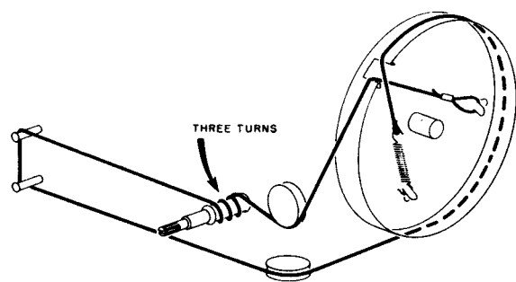
Dial Stringing.
