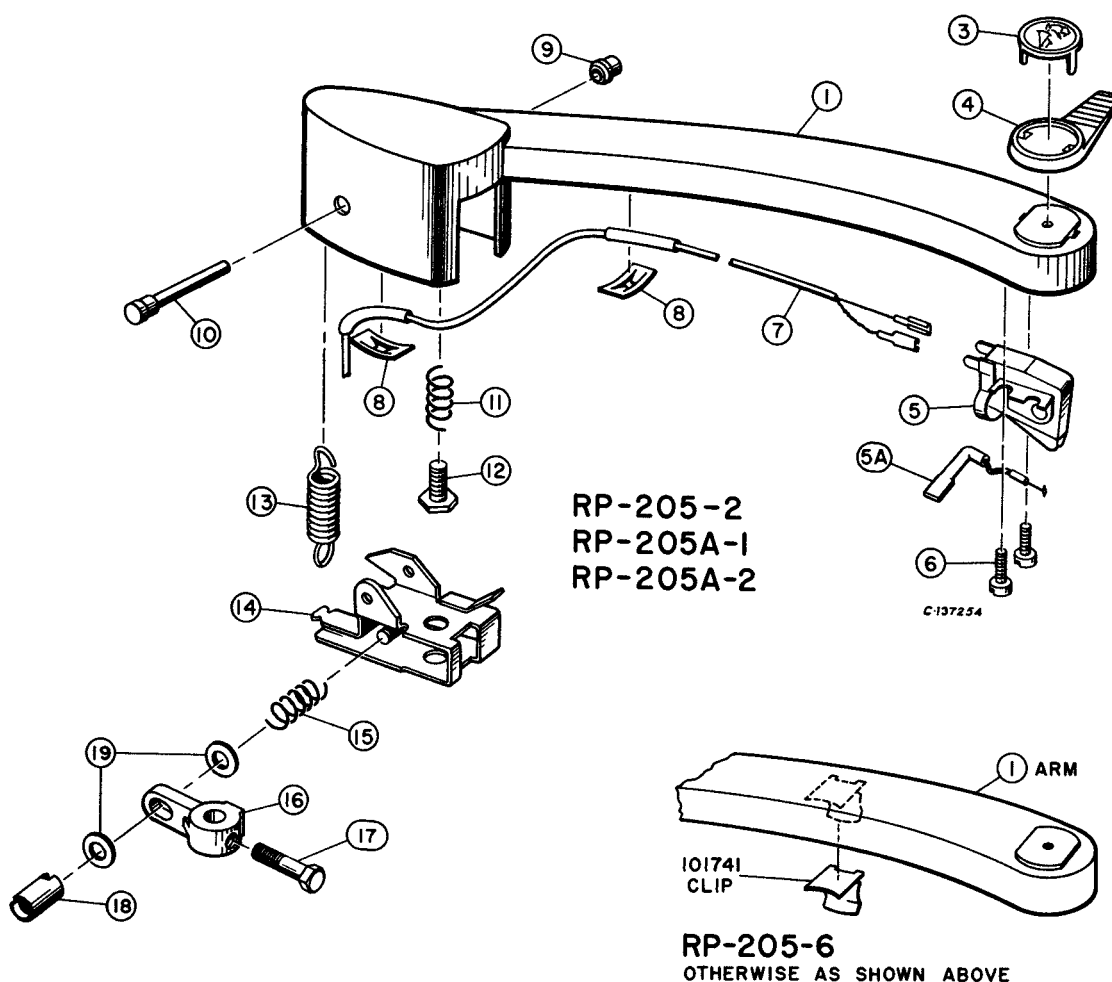
Figure 15—Pickup &amp; Arm Assembly for RP-205-2, RP-205-6, RP-205A-1 and RP-205A-2
