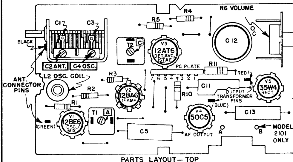
PARTS LAYOUT - TOP
