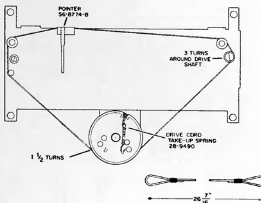
Dial Cord Stringing — Model E-818
