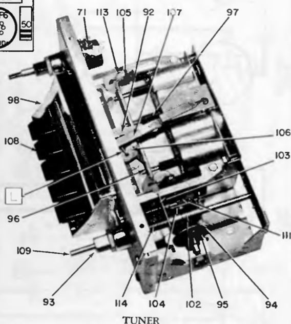
TUNER
