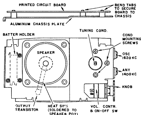
Complete Chassis Assembly
