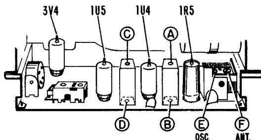
Figure 1. Tube and Adjustment Location.
