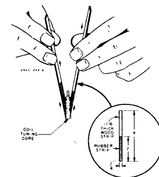
CORE ALIGNMENT TOOL DETAIL
