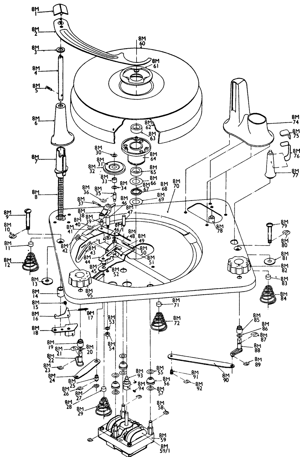
MAINPLATE ASSEMBLY
