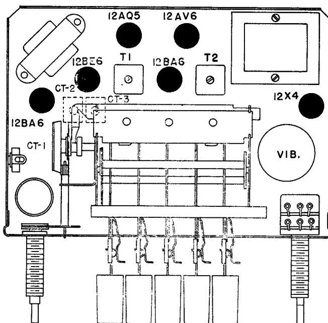
Tube and Trimmer Locations
