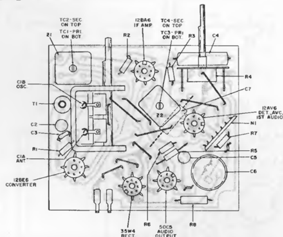
Printed Panel Component Layout—Model E-742
