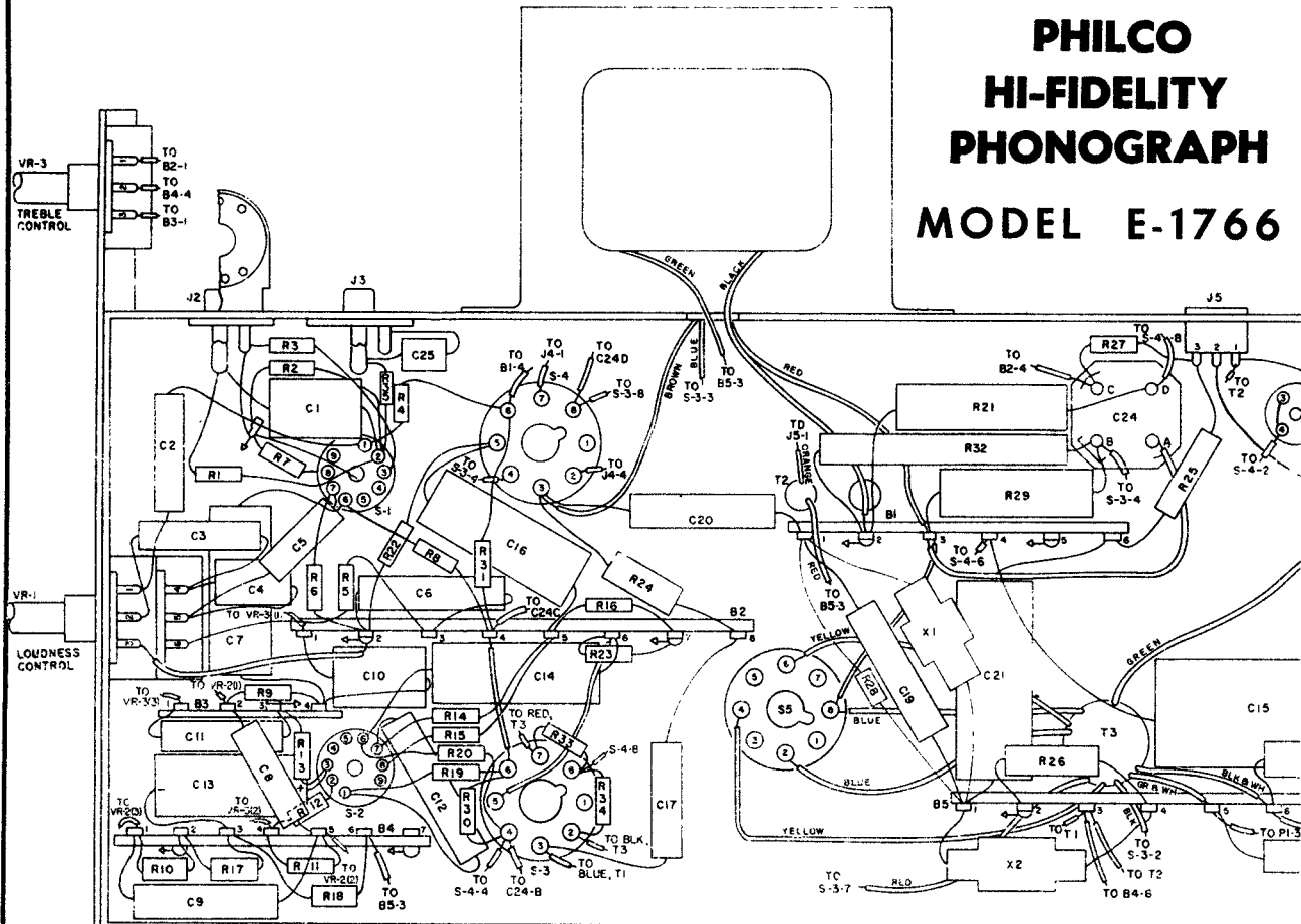
Base View — Model E-1766
