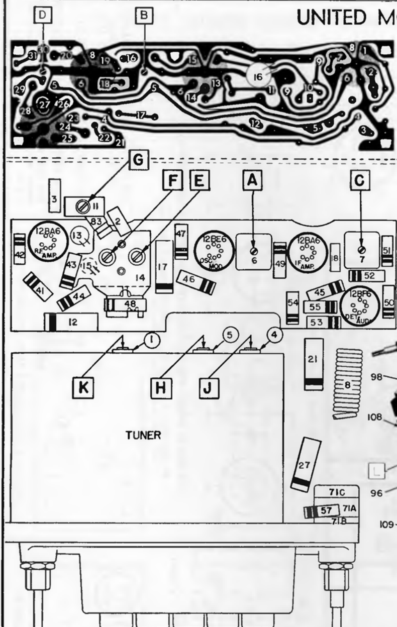
PARTS LAYOUT—TUBE VIEW
