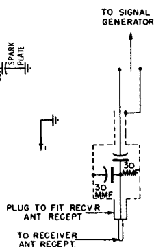
DUMMY ANTENNA DATA
