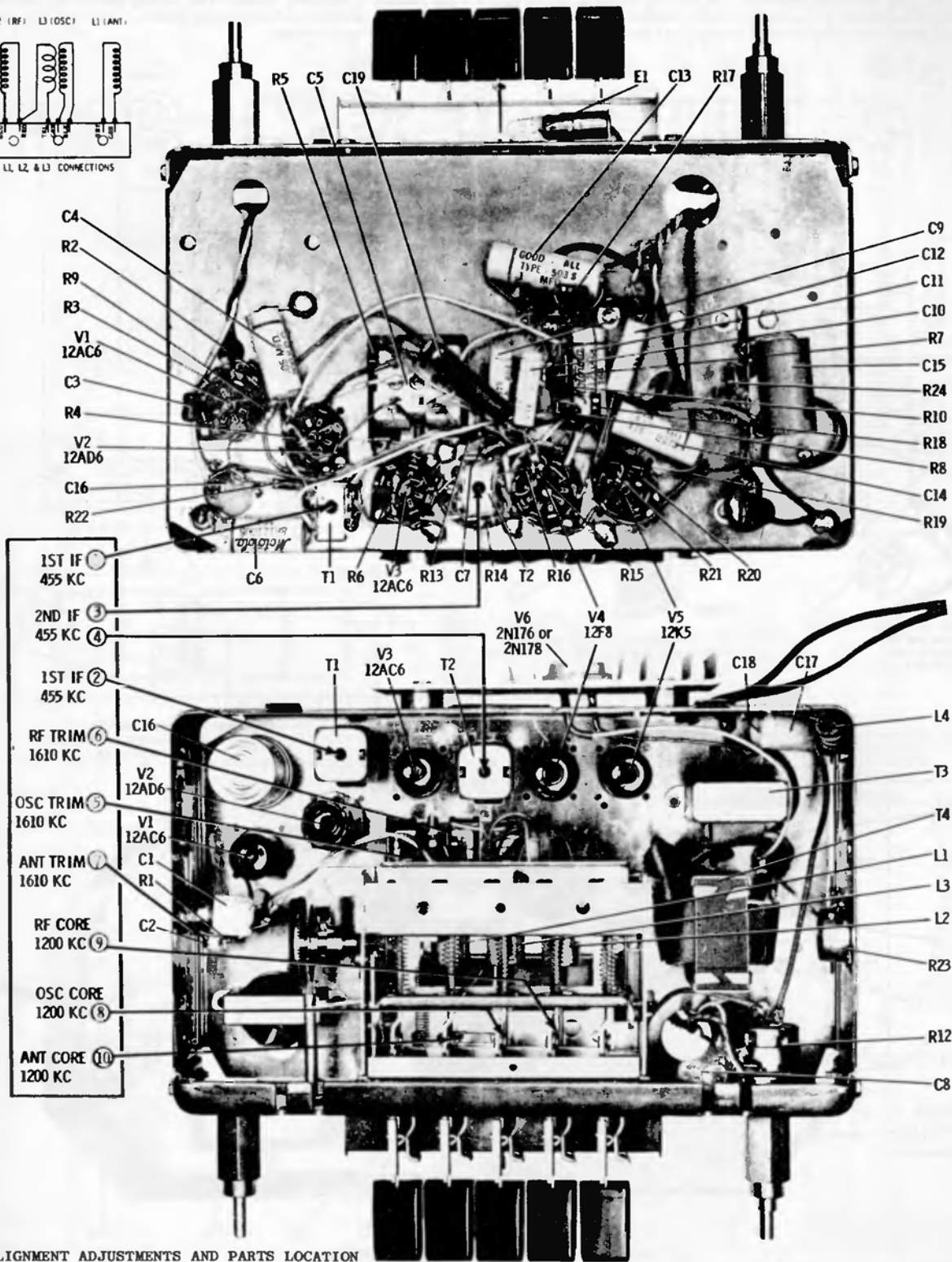
ALIGNMENT ADJUSTMENTS AND PARTS LOCATION
