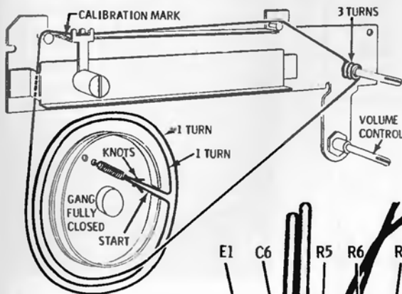
DIAL STRINGING
