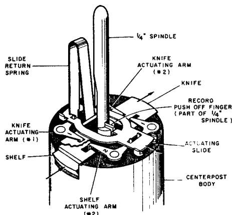
Figure 9—Centerpost Operation
