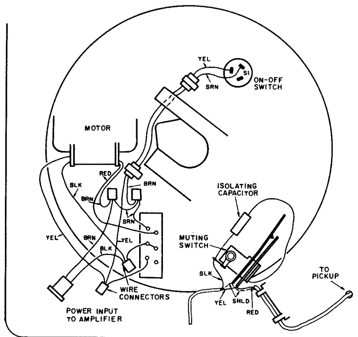
Figure 18—Wiring Diagram for Dual-Voltage Motors
