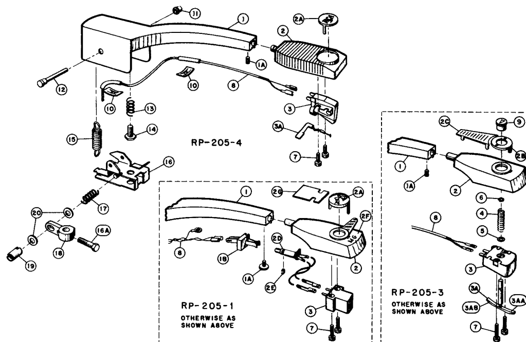
Figure 16—Pickup &amp; Arm Assembly for RP-205-1, RP-205-3 and RP-205-4
