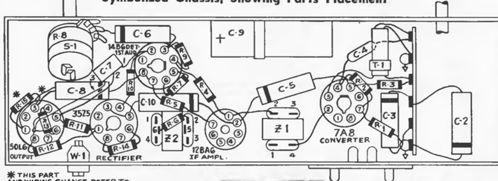
Symbolized Chassis, Showing Parts Placement
