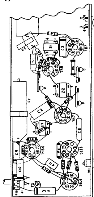
Symbolized Chassis, Showing Parts Placement
