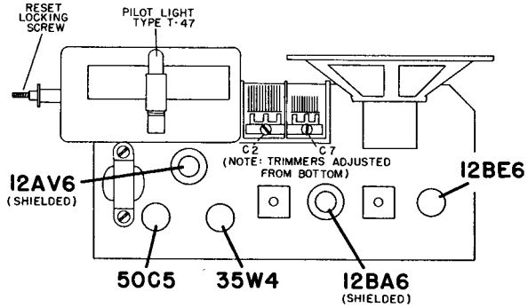
CHASSIS VIEW, SHOWING TUBE LOCATIONS
