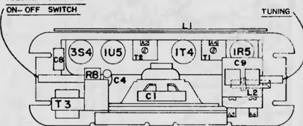
TUBE LAYOUT
