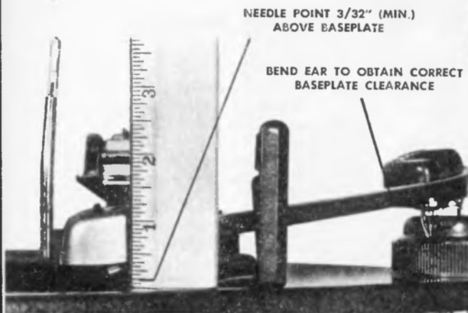
FIGURE 4. BASE-PLATE-CLEARANCE ADJUSTMENT
