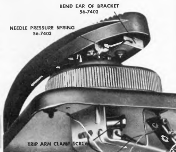
FIGURE 9. NEEDLE-PRESSURE ADJUSTMENT
