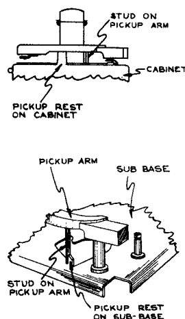
Figure 24—Pickup Arm Rest.
