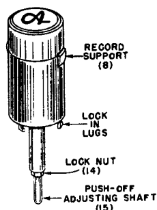
Figure 7. 45 RPM Centerpost.
