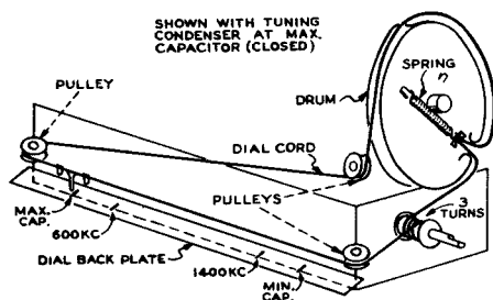
Dial Indicator and Drive Cord
