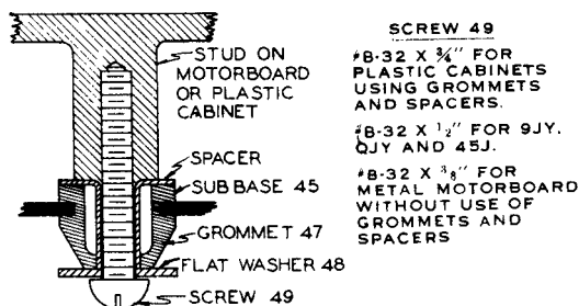
Figure 25—Sub-base Mounting.
