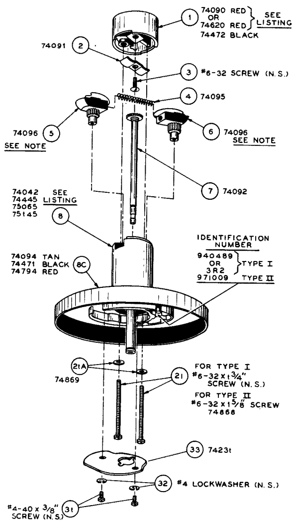
Figure 20: Turntable Assemblies, Types I and II.
