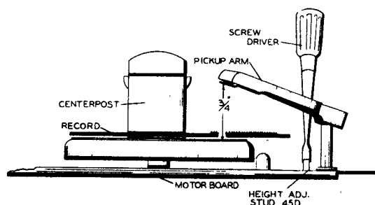
Figure 41—Height Adjustment.
