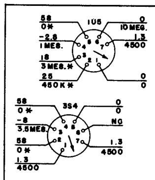
Voltage and Resistance Diagrams, Chassis 120112
