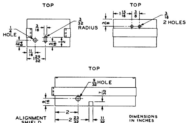
Fig. 3—Alignment Shield
