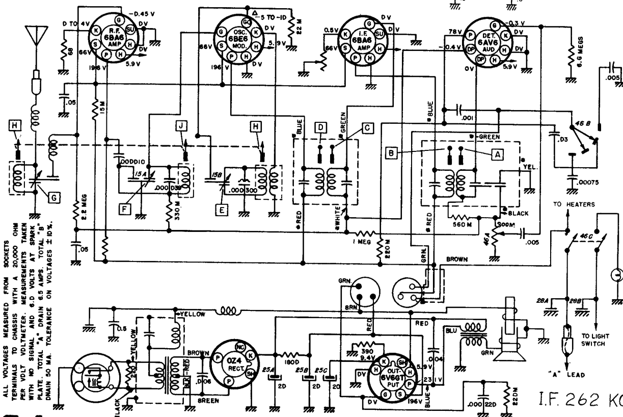
CIRCUIT DIAGRAM—RADIO 986240 and 986388
