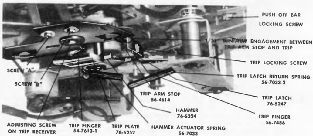
FIGURE 3. TRIP ADJUSTMENTS
