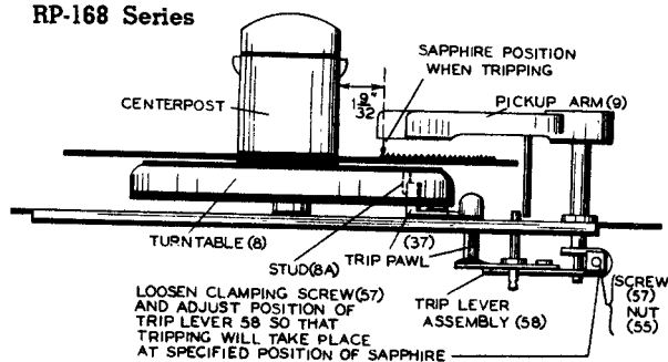
Figure 39—Tripping Position.
