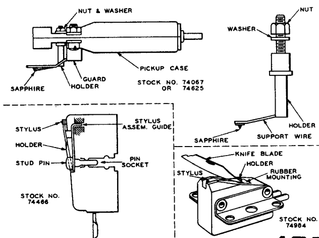
Figure 16—Stylus Replacement.
