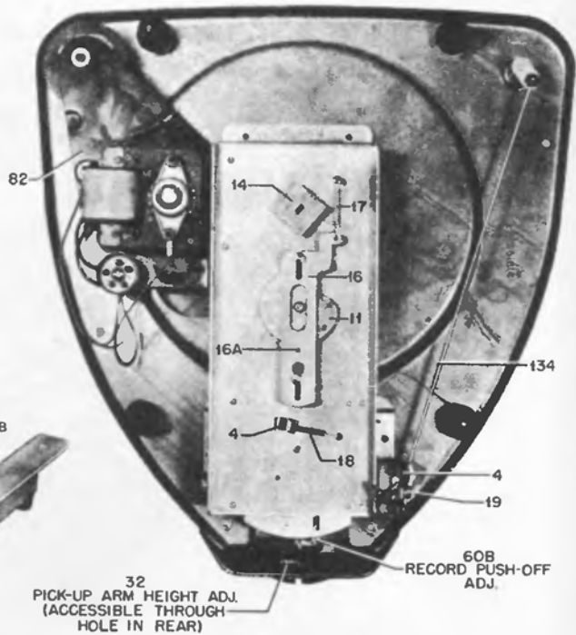
FIGURE 4. BOTTOM VIEW OF RECORD CHANGER
