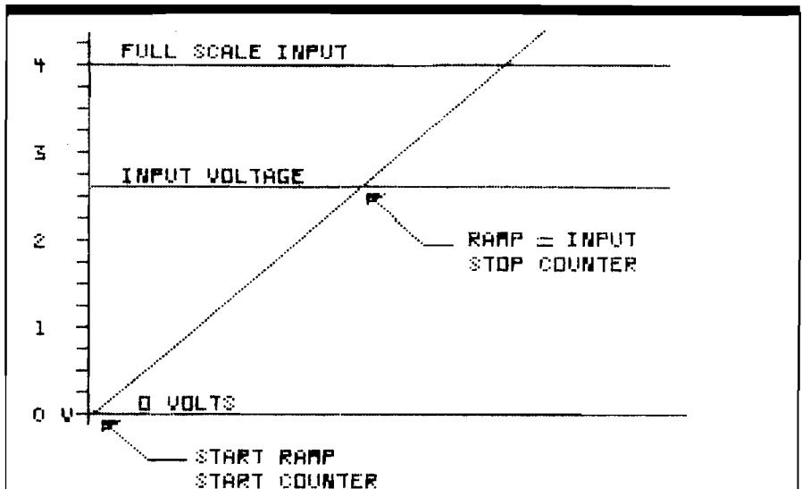
Figure 1. Operating scheme for a single-slope A/D converter.
