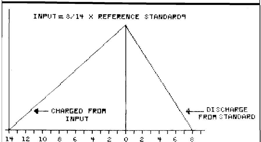
Figure 2. Operating concept of a dual-slope integrating A/D converter. A capacitor is charged by the input voltage for a fixed time, then discharged by a reference source. The input voltage is determined by a ratio of charge to discharge times.
