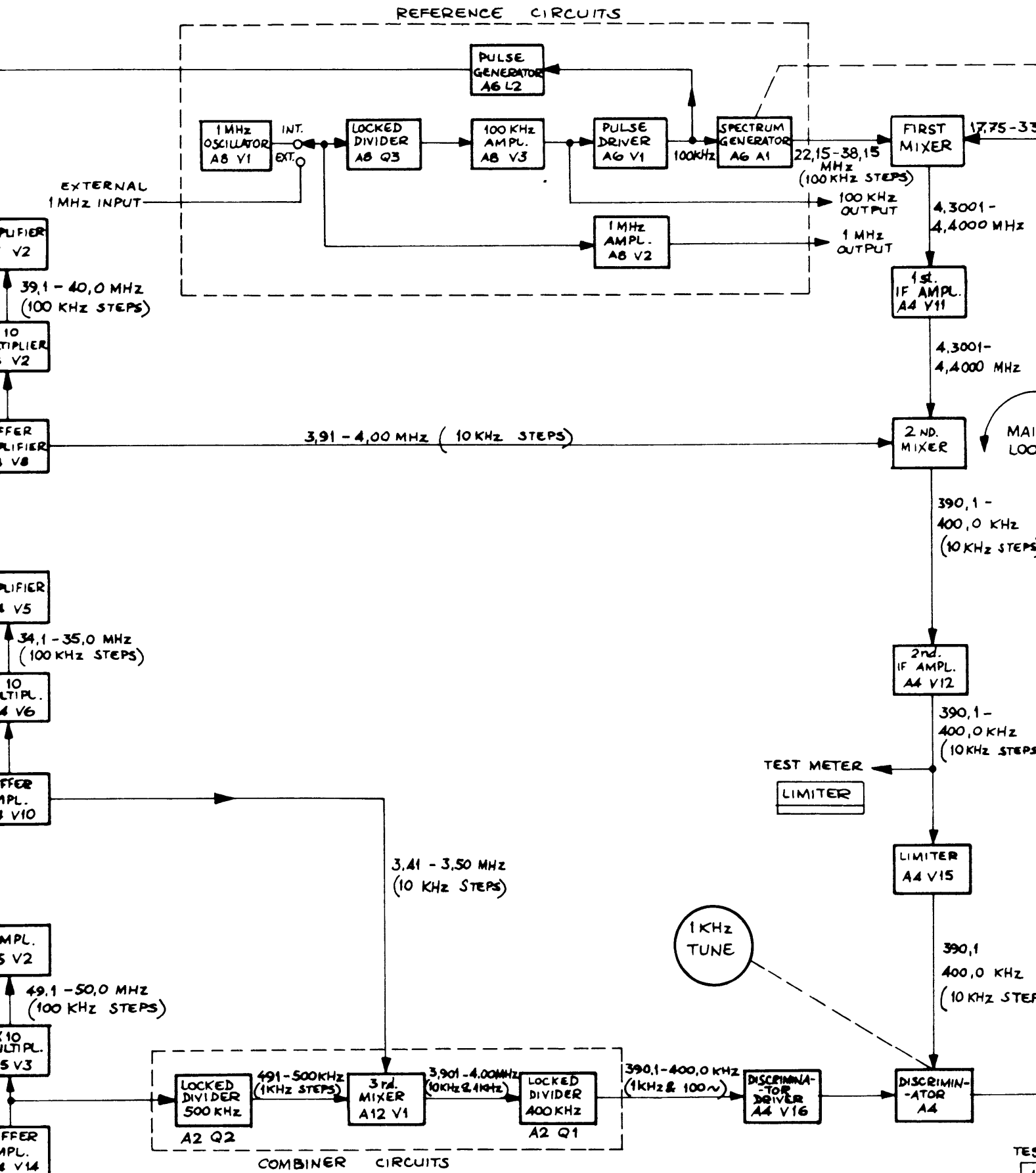
Fig. 1 - HALLICRAFTER SYNTHESIZER
