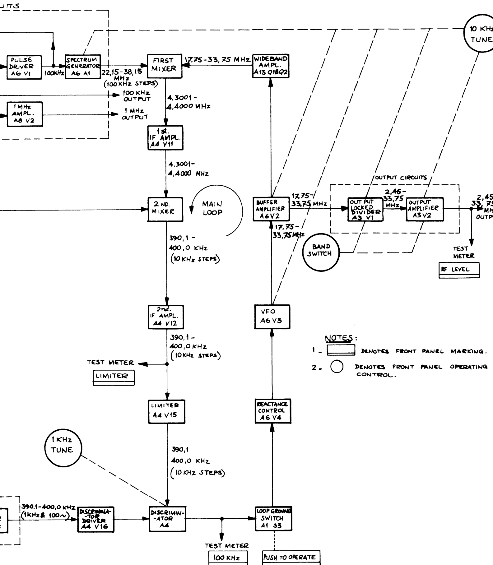
Fig. 1 - HALLICRAFTER SYNTHESIZER BLOCK DIAGRAM (MODEL MHS-402)
